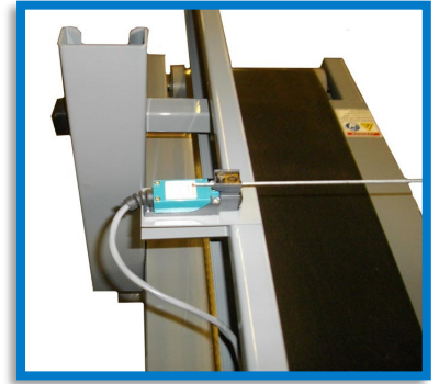
Start/Stop Wand Switch
